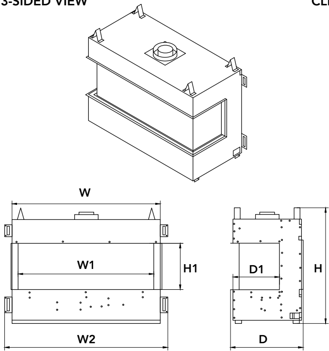
3-SIDED VIEW
